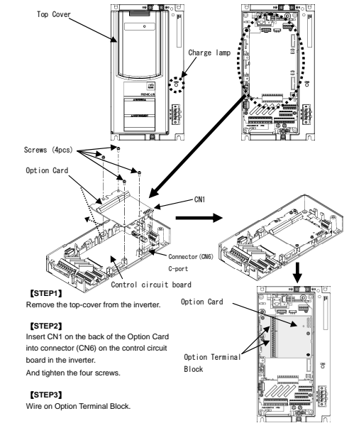
Figure 1.2 Installation Drawing
