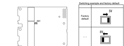
Figure 5.4 Location of the Slide Switch on OPC-PSH
